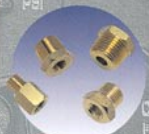
adaptor 543-31 1/8 NPT x 1/8 BSP elec water temp adaptor 543-32 1/8 NPT x 3/8" NPT elec water temp adaptor 543-33 1/8 NPT x 1/2" NPT elec water temp adaptor 543-34 1/8 NPT x 3/8" UNF elec water temp
